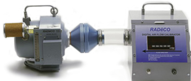
Calibration Set Up
